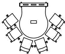
MODEL # SM-TR-4660 54" X 60" - 6 CHAIRS
